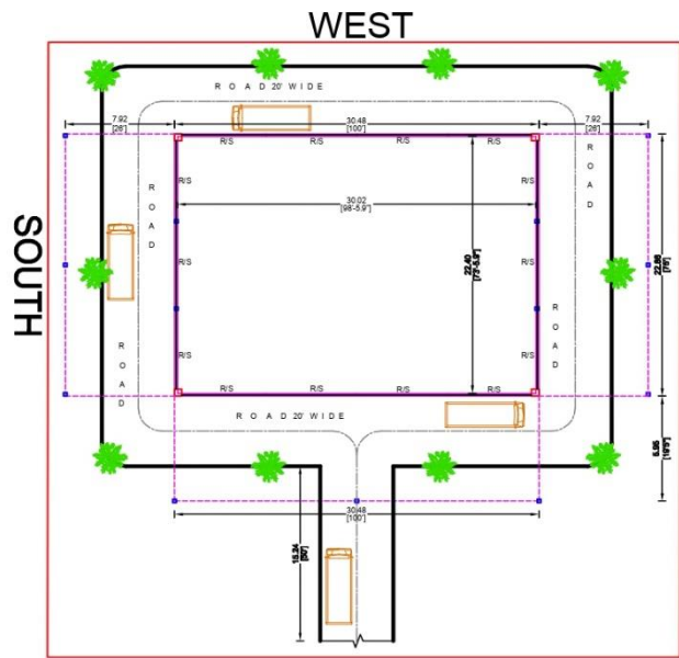
EAST PLAN
