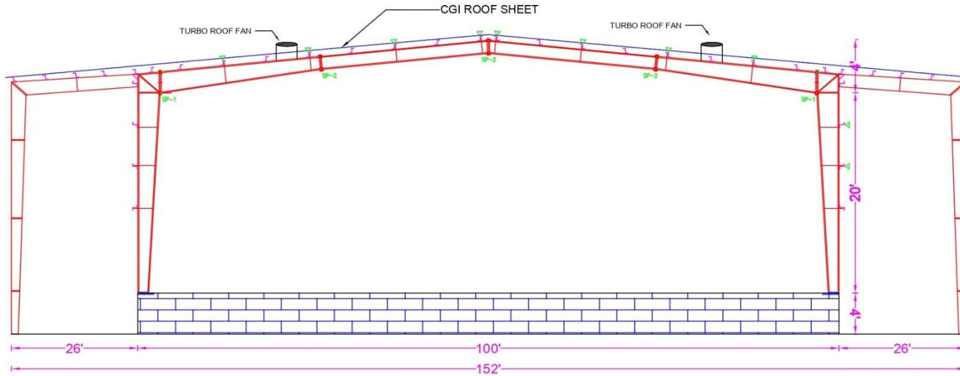
SECTION
