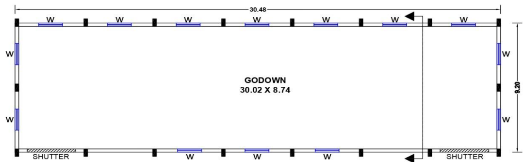
PLAN
